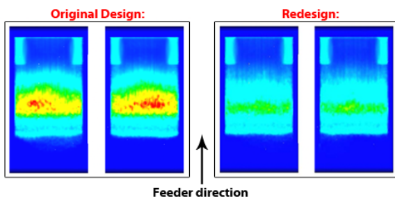
Figure 3: DEM impact intensity contours of the two feeder belts: Left: Initial situation, Right: with inclusion of TBS designed baffles
