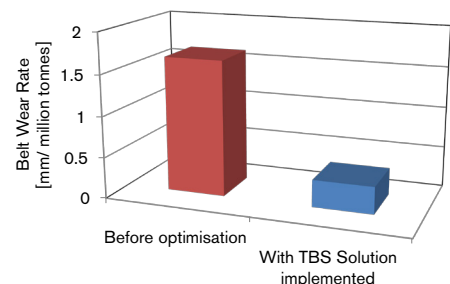
Figure 4: Decrease in belt wear rate after optimisation
